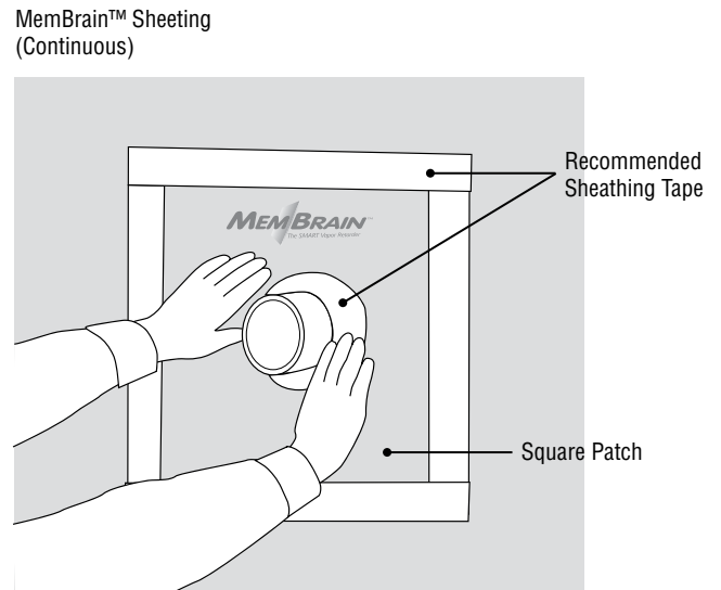
Figure 11: Patch attachment.
