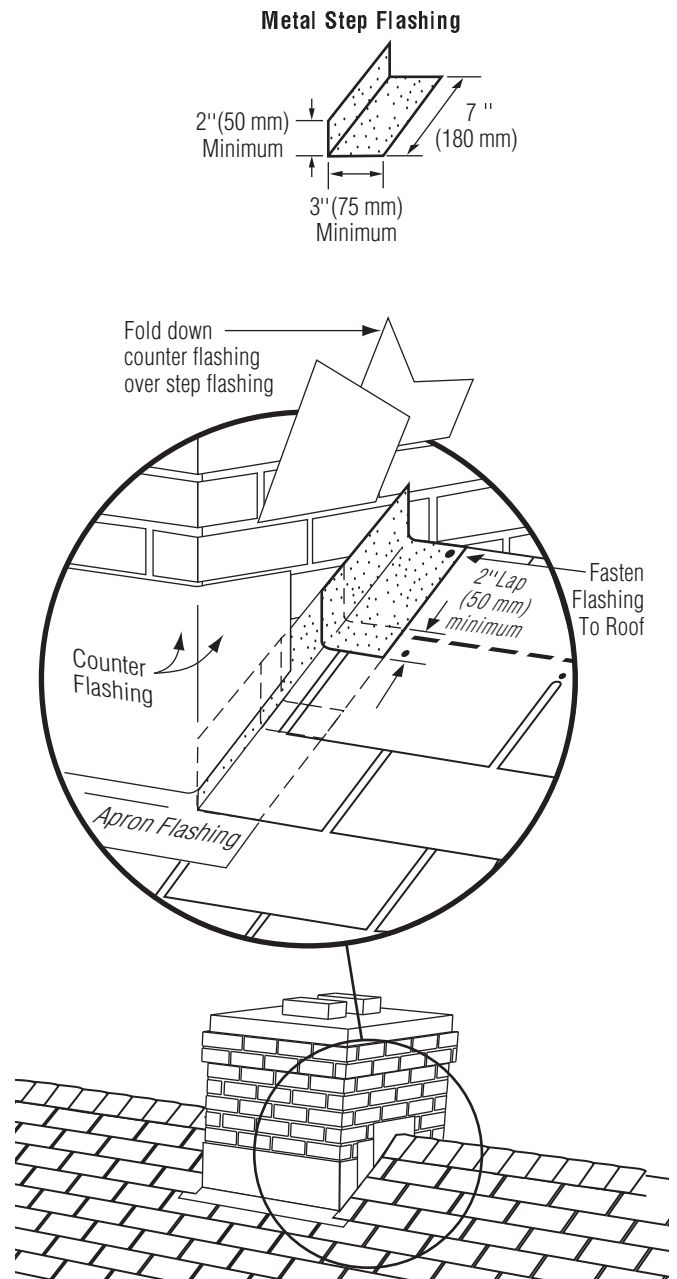
Figure 10-18: Flashing around a chimney.
