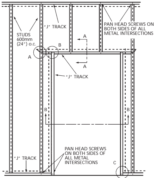
DUCT OPENING ROOM SIDE
