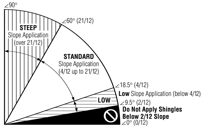
Figure 16-2: Slope definitions.
