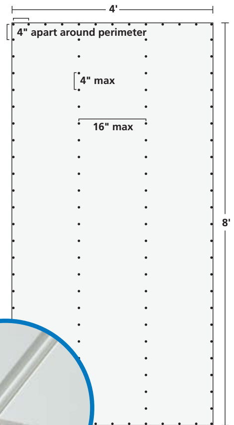
Fastening Diagram
