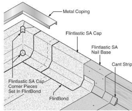
Figure 5-40: Inside Corner 2 Ply System
