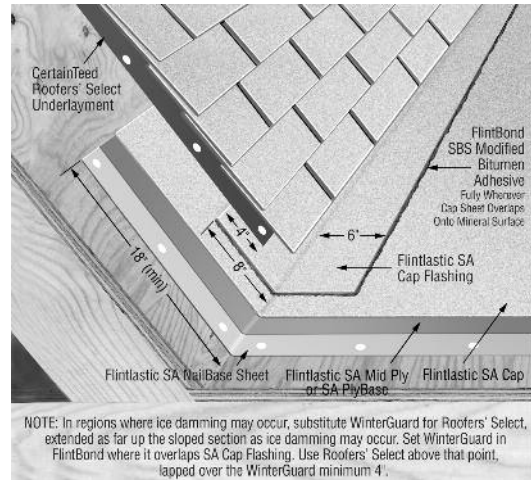
Figure 5-34 Shingle Transition 3 Ply
