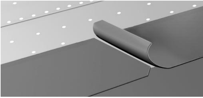
Figure 5-17: Cut endlaps at a 45 degree angle at opposing diagonal corners.
