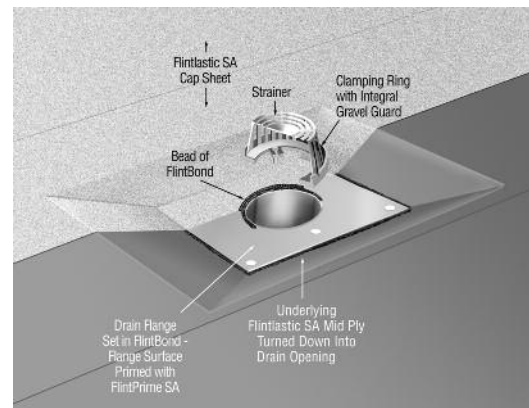
Figure 5-36: Drain 3 Ply
