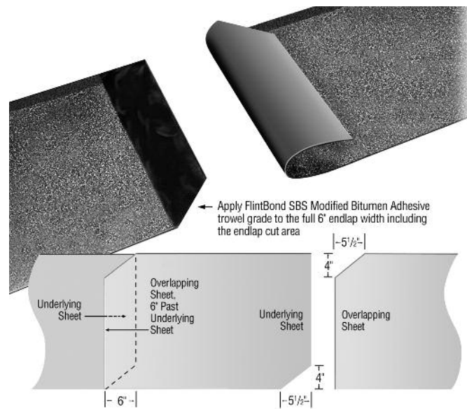
Figure 5-24: Trim the corners of the underlying and overlapping sheets as shown.
