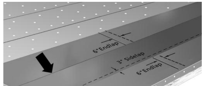
Figure 5-16: Roll seams with a heavy weighted roller.
