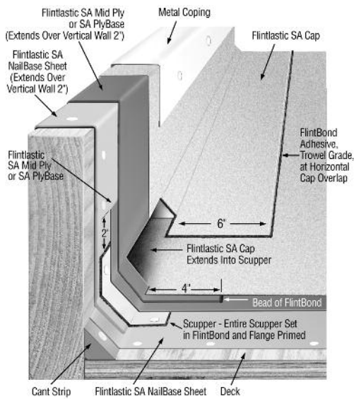
Figure 5-38: Scupper 3 Ply
