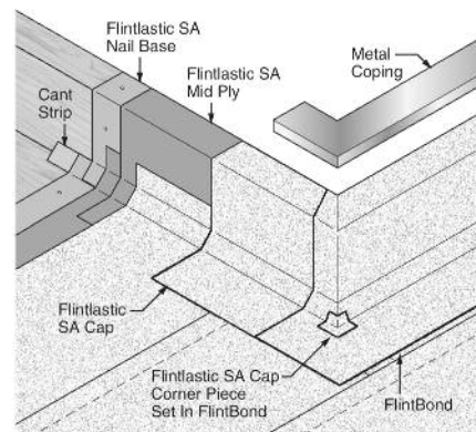
Figure 5-43: Outside Corner 3 Ply System
