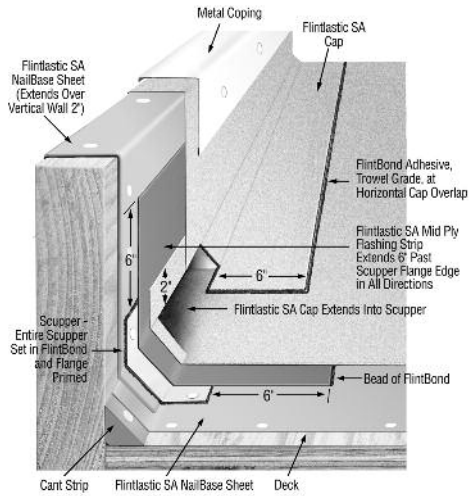
Figure 5-31: Scupper 2 Ply
