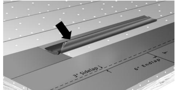
Figure 5-15: Fold back halfway and remove release film.
