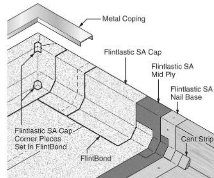
Figure 5-41: Inside Corner 3 Ply System
