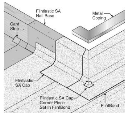
Figure 5-42: Outside Corner 2 Ply System
