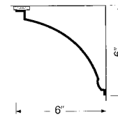
60806 Cornice 6" Projection 6" Deep 48" Long
