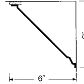
60904 Cornice 6" Projection 6" Deep 48" Long
