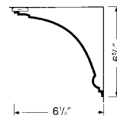
60707 Cornice 6 1/4" Projection 6 5/8" Deep 48" Long
