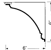
60906 Cornice 6" Projection 6" Deep 48" Long
