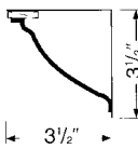
60802 Cornice 3 1/2" Projection 3 1/2" Deep 48" Long
